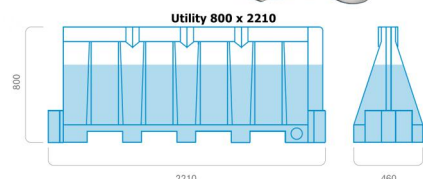
Utility 800 x 2210
