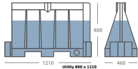
Utility 800 x 1210
