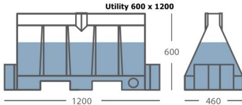
Utility 600 x 1200
