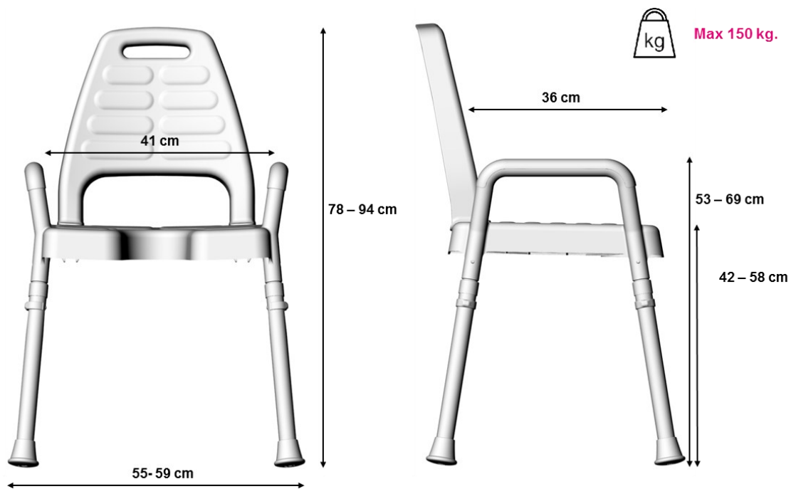
Nielsen Line Shower stool 41 cm.
