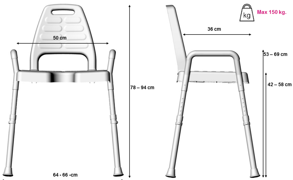
Nielsen Line shower stool 50 cm.
