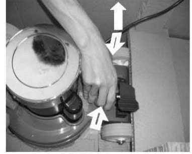
Step 3 - Press both sides of screw box inwards and pull it out
