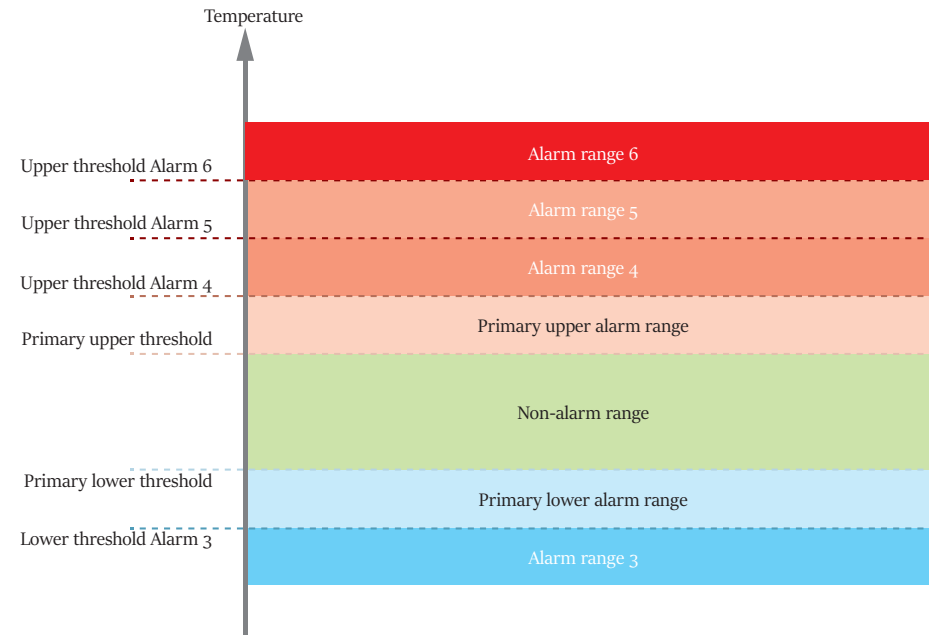
Figure 40: Alarm ranges for USRIC-8M
