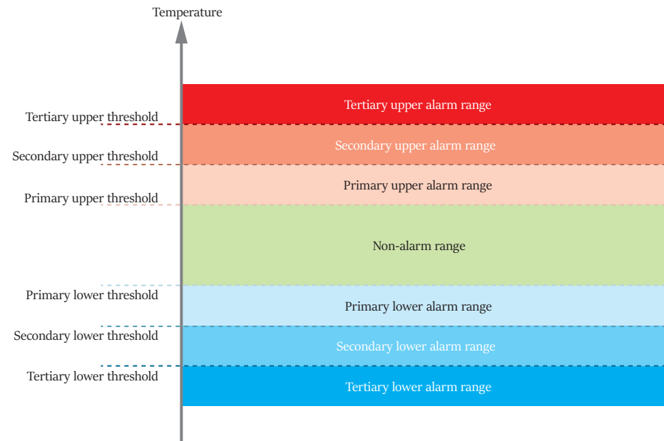
Figure 42: Alarm ranges for UTRID-16
