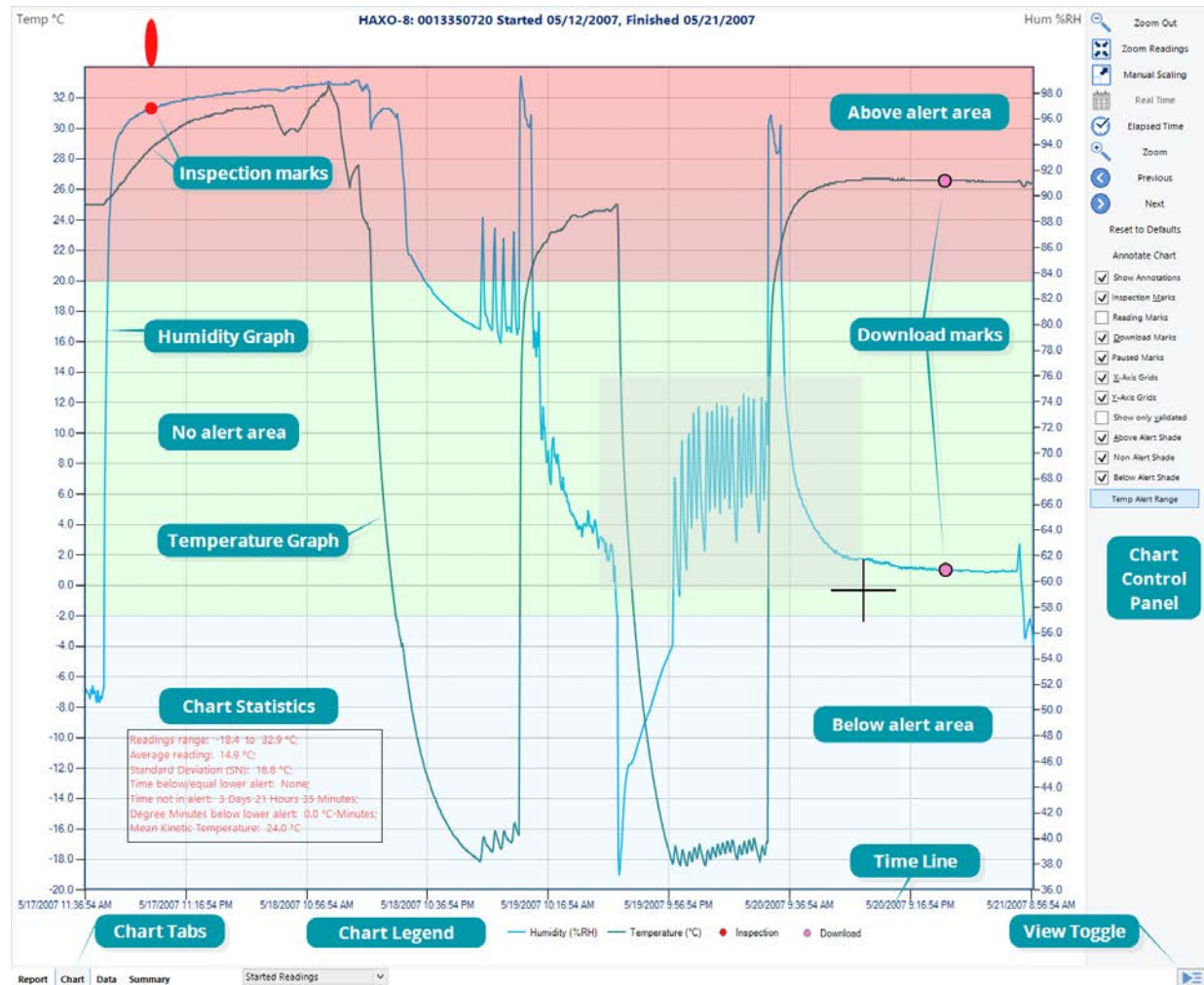
Figure 66: Chart display
