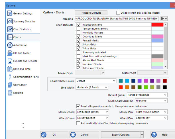
Figure 107: Chart options
