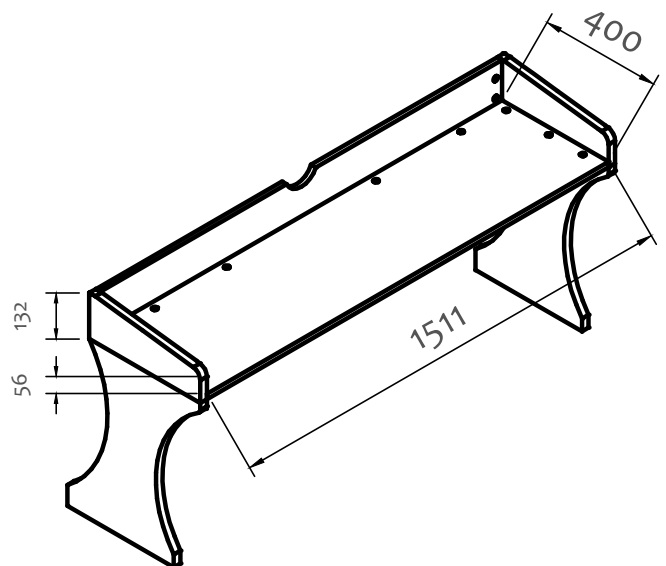
KEYBOARD TRAY
