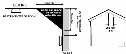
Figure 3i- Positioning the smoke /heat detector Figure 3ii
