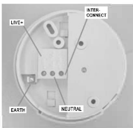
Figure 5 –Wiring & Interconnect facility
