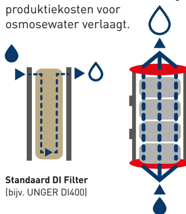
HydroPower® DI filter HOGERE EFFICIENCY
