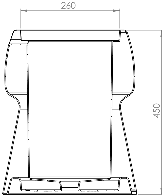
SECTION VIEW
