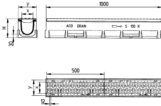
Gootelement, 1 meter, S100K, S150K, S200K
