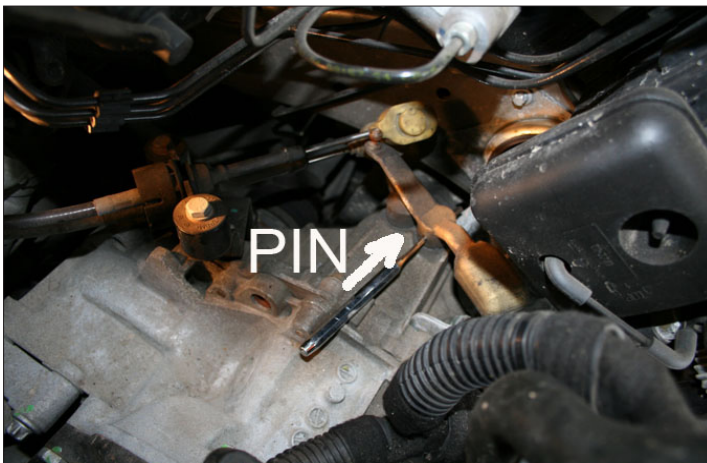
Use a punch tool and a hammer to remove locking pin.
