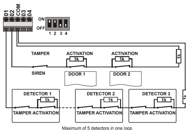
Maximum of 5 detectors in one loop
